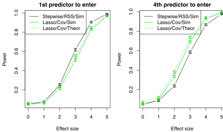
FIG. 4. Estimated power curves for significance tests using forward stepwise regression and the drop in RSS statistic, as well as the lasso and the covariance statistic. The results are averaged over 1000 simulations with n = 100 and p = 10 predictors drawn i.i.d. from N(0, 1) and \sigma^2 = 1 . On the left, there is one truly nonzero regression coefficient, and we varied its magnitude (the effect size parameter on the x-axis). We examined the first step of the forward stepwise and lasso procedures. On the right, in addition to a nonzero coefficient with varying effect size (on the x-axis), there are 3 additional large coefficients in the true model. We examined the 4th step in forward stepwise and the lasso, after the 3 strong variables have been entered. For the power curves in both panels, we use simulation-based cutpoints for forward stepwise to control the type I error at the 5% level; for the lasso we do the same, but also display the results for the theoretically-based [Exp(1)] cutpoint. Note that in practice, simulation-based cutpoints would not typically be available.
